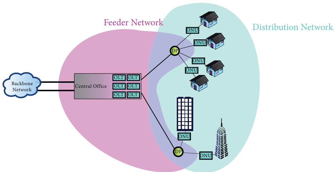
Figure 1.1.3: A passive optical network (PON)
