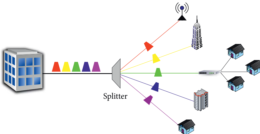
Figure 1.1.4: Standard WDM-PON architecture
