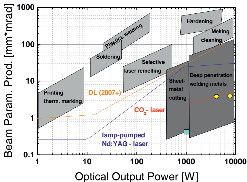
Figure 1.3: Materials processing laser 'roadmap', adapted from [3]. Beam parameter product (BPP) plotted versus optical output power in double-logarithmic scale. The laser source radiance B increases at higher powers and reduced BPP. Relevant laser applications and performance of different laser species are noted. Today the highest radiance is achieved by disk lasers (Trumpf 'TruDisk' series, yellow dots) and fiber lasers (IPG 'YLR-1000WC', blue rectangle).
