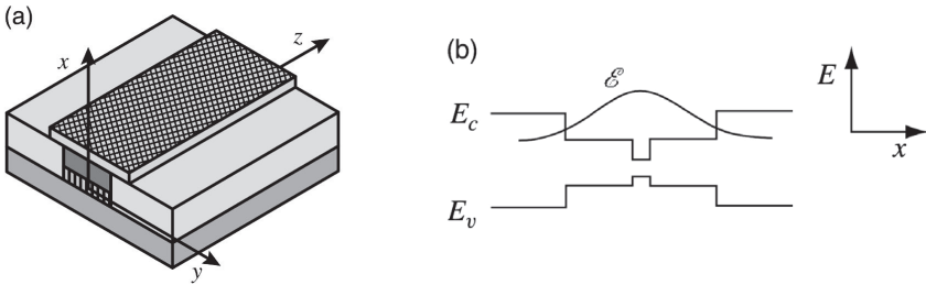
Figure 2.1: (a) Schematic setup of an edge emitting diode laser. (b) Transverse band structures for a standard separate confinement heterostructure. Figures taken from [Col98].
