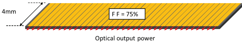
Figure 1.2: Schematic lateral layout of a high fill factor bar.
