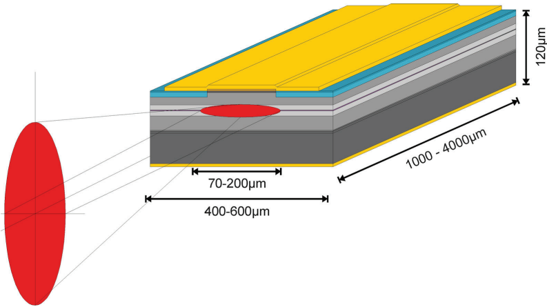
Figure 2.3: Schematics and dimensions of a high power single emitter broad area laser.
