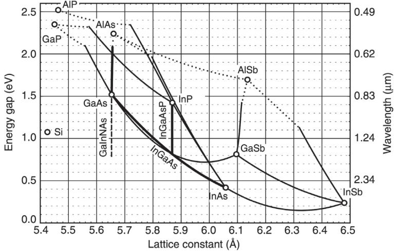
Figure 2.2: Bandgap energy plotted against lattice constant for III-V semiconductors. The single points are binary compounds, with the curves representing ternary compounds with direct (solid) and indirect (dashed) bandgaps. Figure taken from [Col98].
