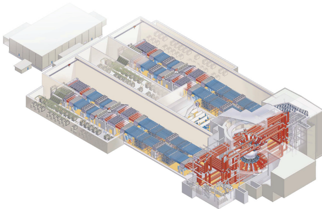
Figure 1.1: Schematic layout of the 192 beamlines and the target chamber at the National Ignition Facility. Figure taken from [NIF16].
