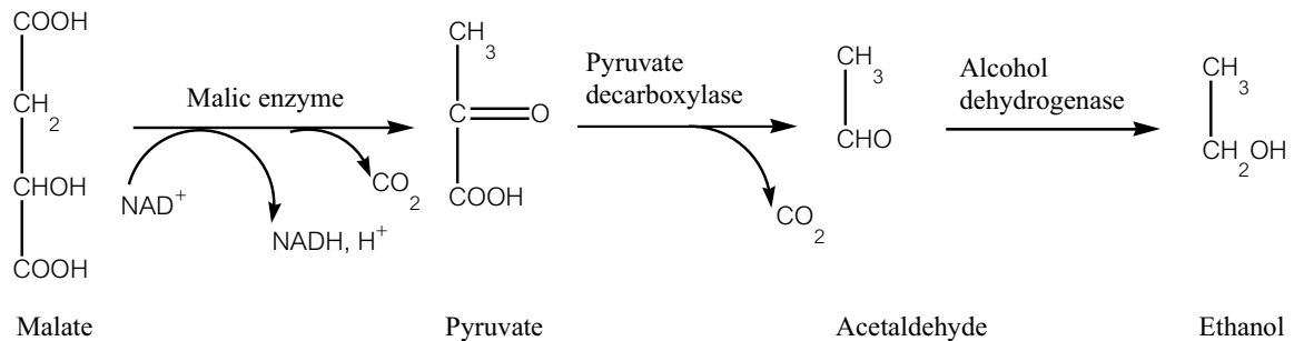
Figure 1.3 Decomposition of malic acid by yeasts during alcoholic fermentation (Ribéreau-Gayon et al., 2000a).
