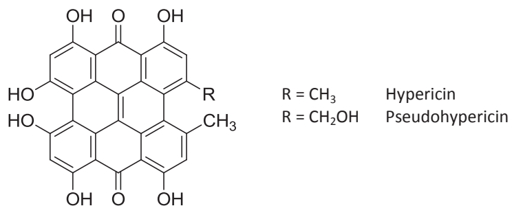
Abb. 7 Hypericine
